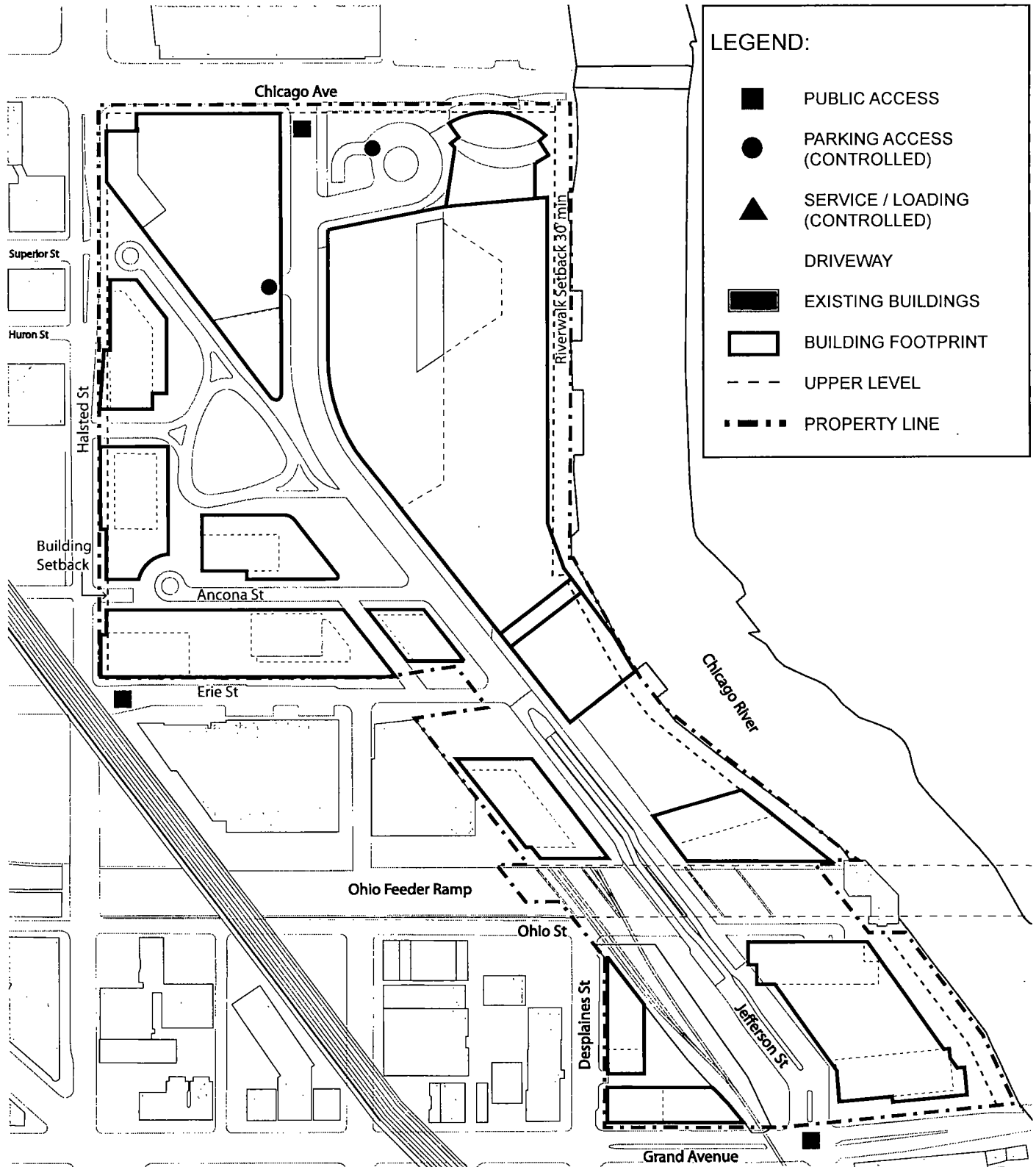
SITE ACCESS AND LOADING PLAN LEVEL 2 (+38.0 TO +45.0 CCD)
