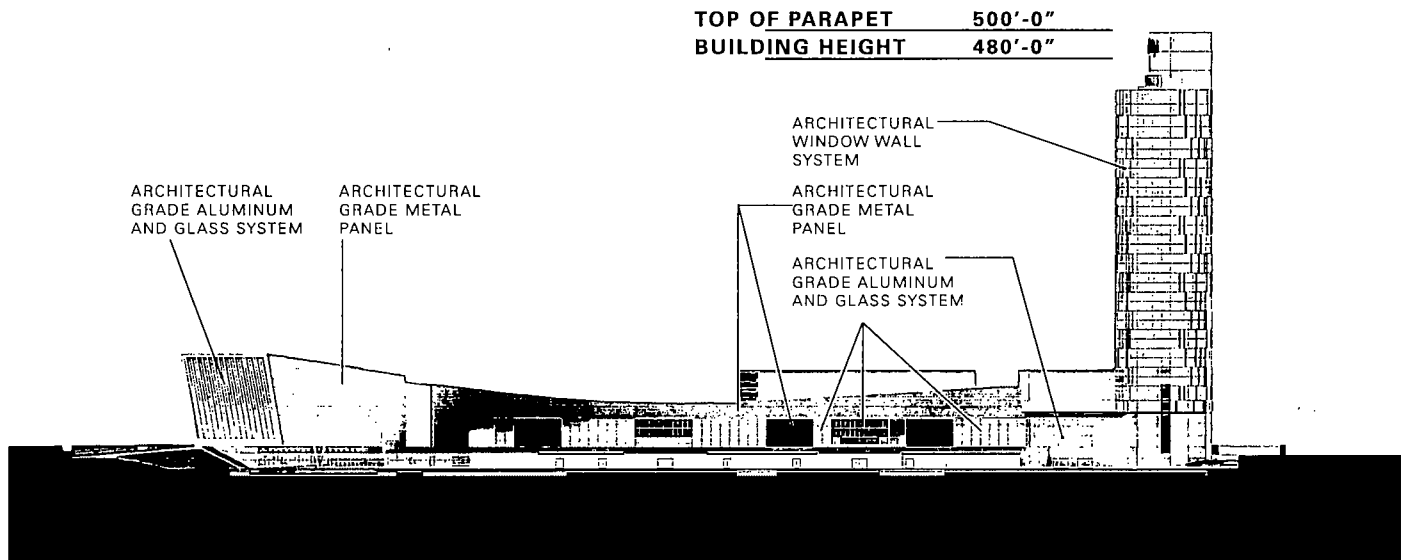
EAST ELEVATION
