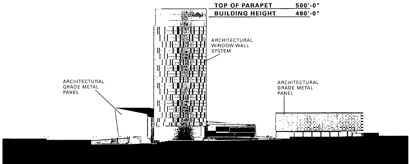
NORTH ELEVATION
