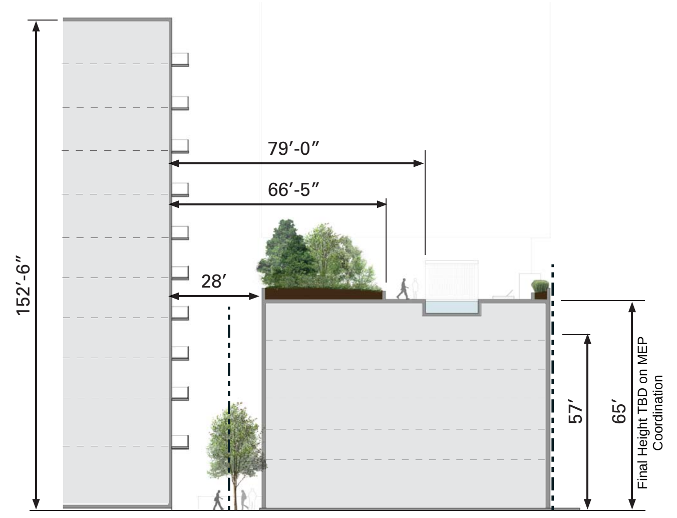
SECTION C
