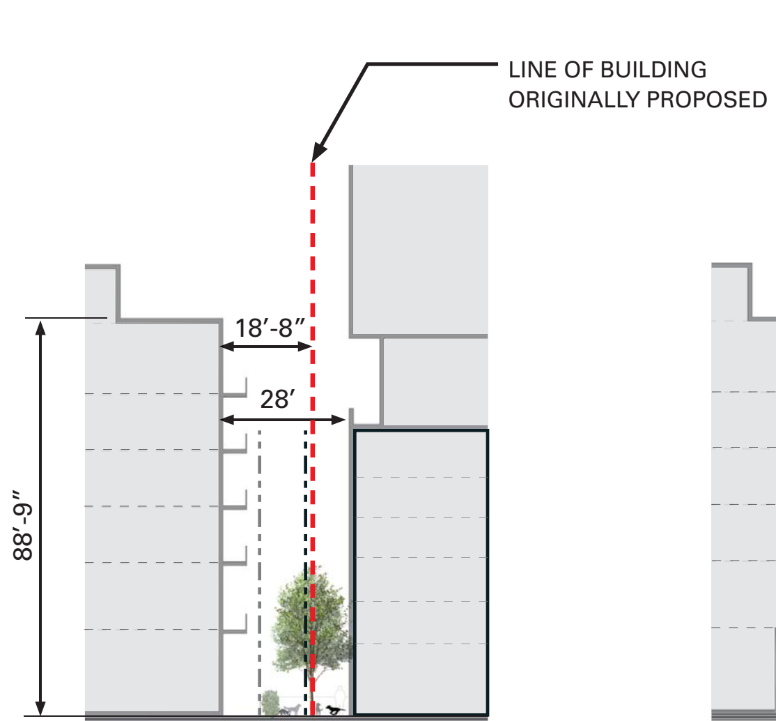
SECTION B
