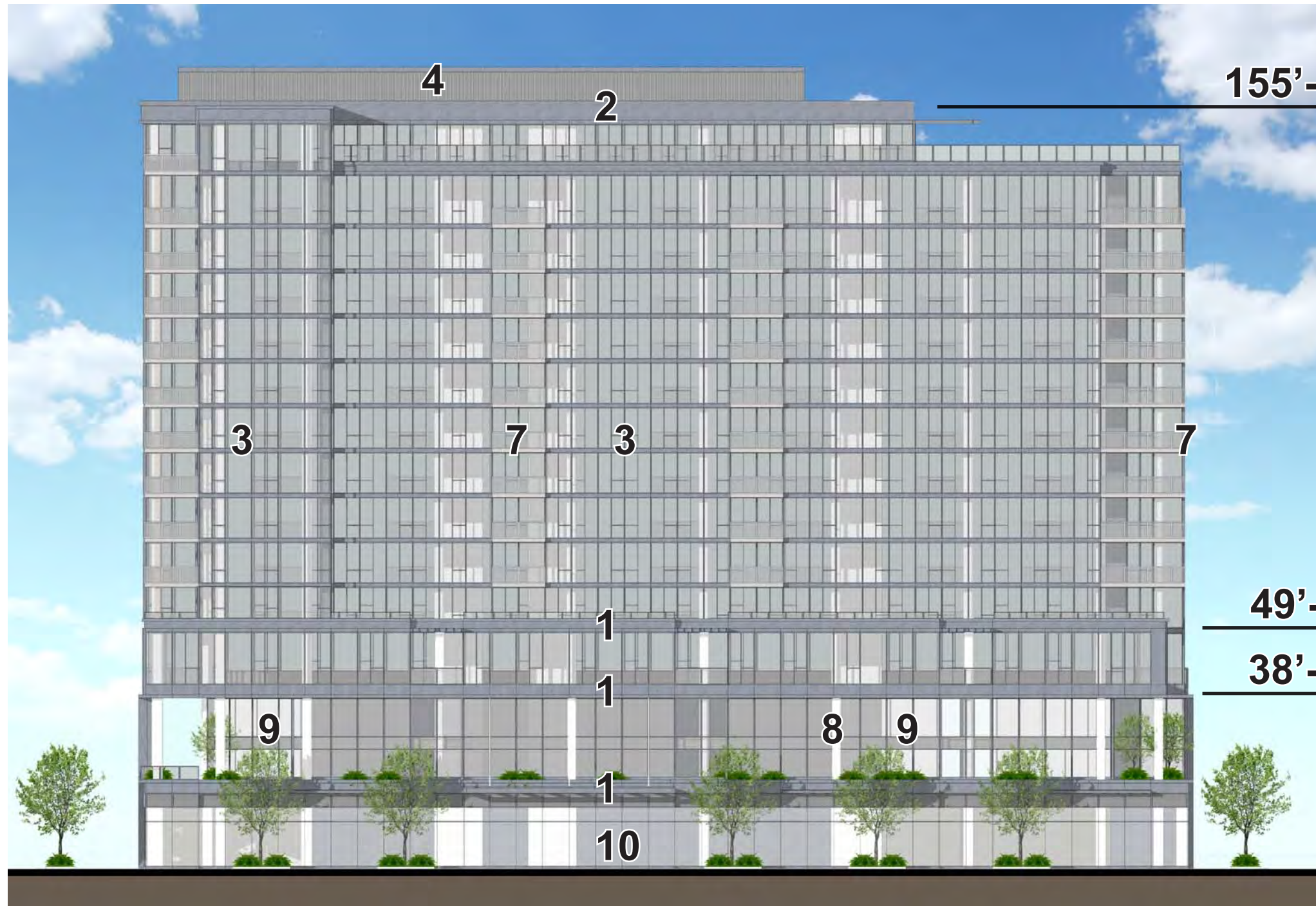
west elevation
